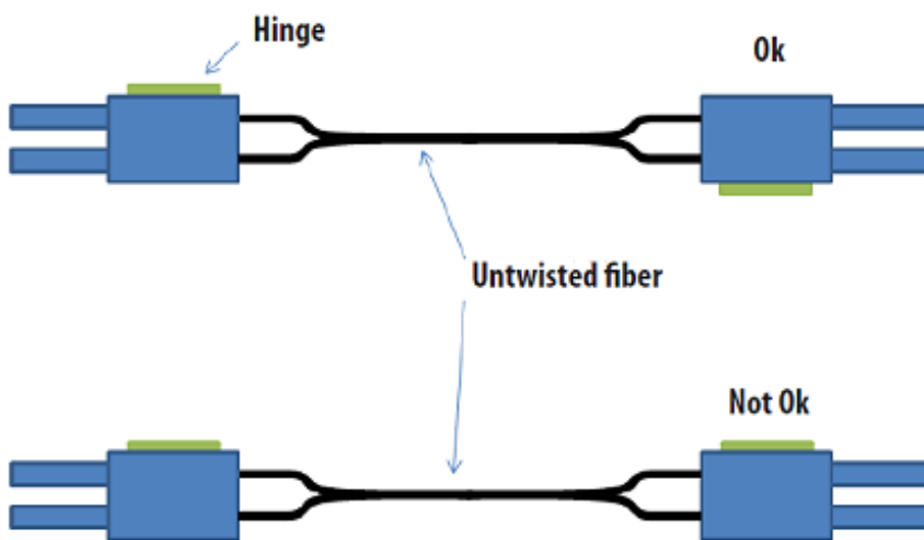
Fig. 56: Correctly connected optical channels
